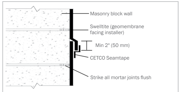
Figure 13 - Masonry wall joint detail
