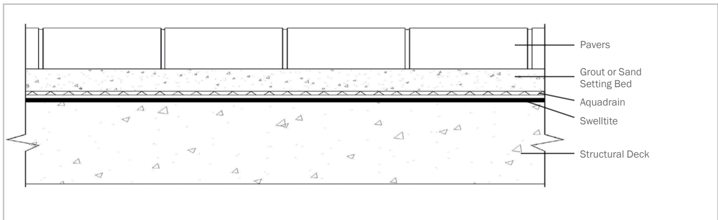
Figure 4 - Typical paver plaza deck detail
